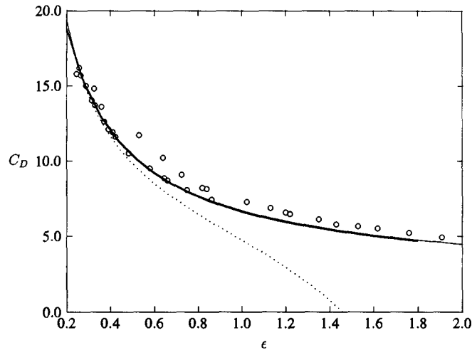
Fig. 7. The hybrid result (3.26) for C_D without the O(\epsilon^2) term (solid line) is compared with experimental results (discrete points), with full numerical results (heavy solid line) and with the two-term result C_D \sim 4\pi\epsilon^{-1}(\delta - 0.8669\delta^3) (dotted line). Notice that the hybrid results and the full numerical results for C_D are virtually indistinguishable.
