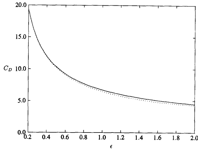
Fig. 8. The hybrid result (3.26) for C_D without the O(\epsilon^2) term (solid line) is compared with the hybrid result (3.26) with the O(\epsilon^2) term (dotted line).
